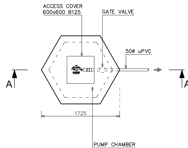
LAYOUT PLAN
