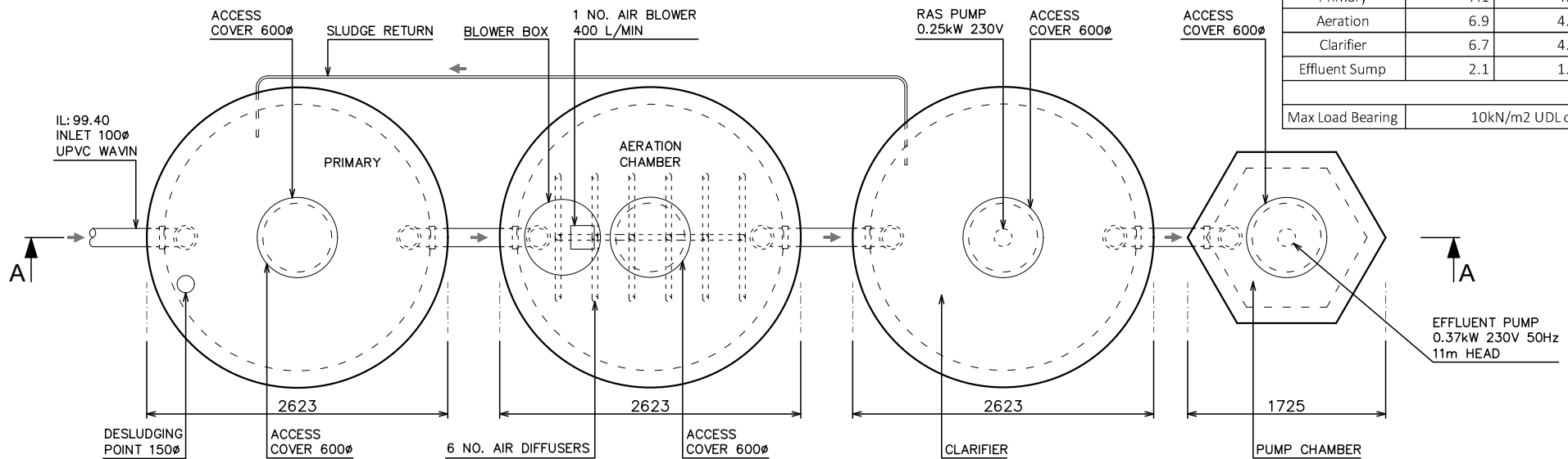
LAYOUT PLAN
