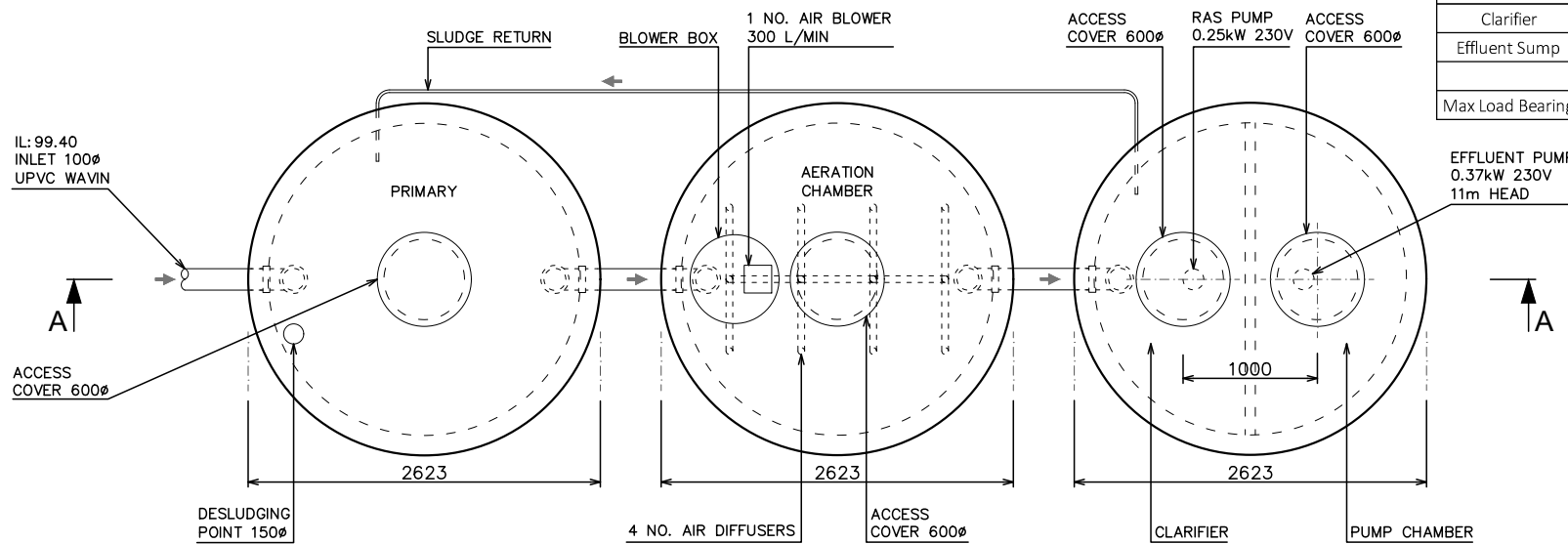
LAYOUT PLAN
