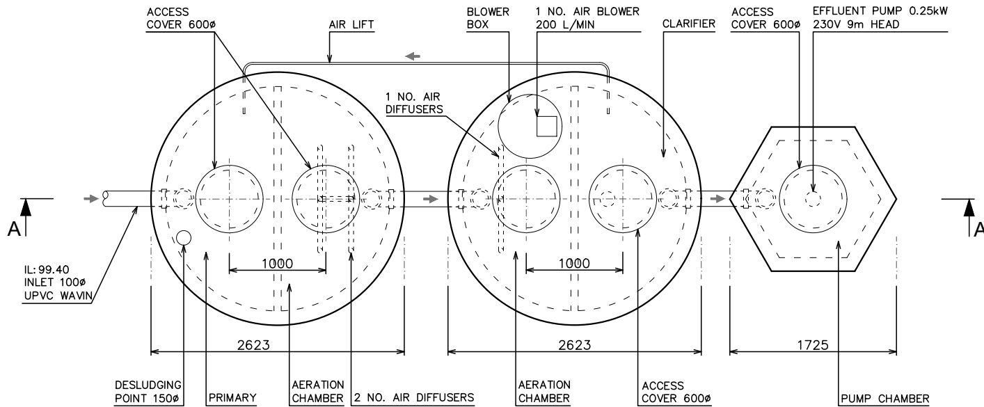
LAYOUT PLAN
