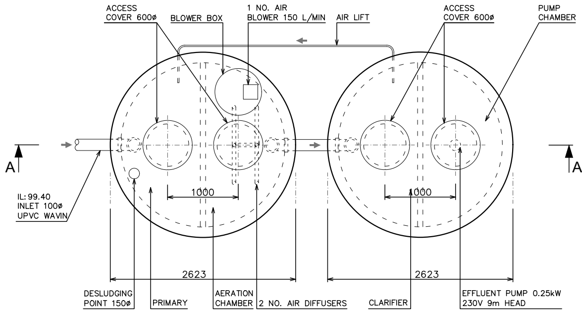
LAYOUT PLAN
