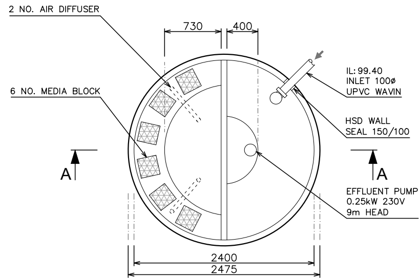
TANK PLAN
