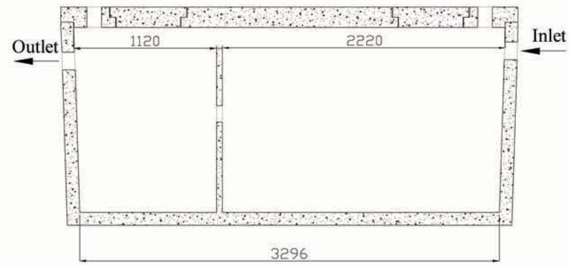
Cross Section
