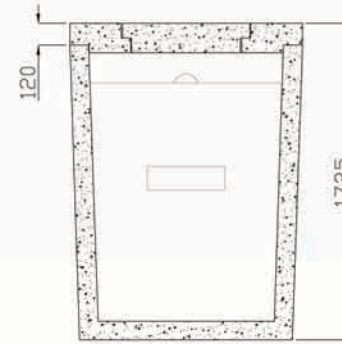
Vertical Section
